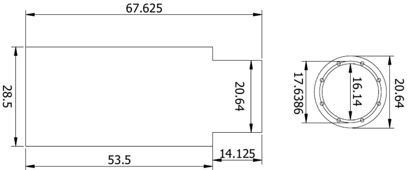
Figure 3: The dimensions of the feed support cylinder in inch are shown in the diagram. The cryostat will be located within this cylinder.
