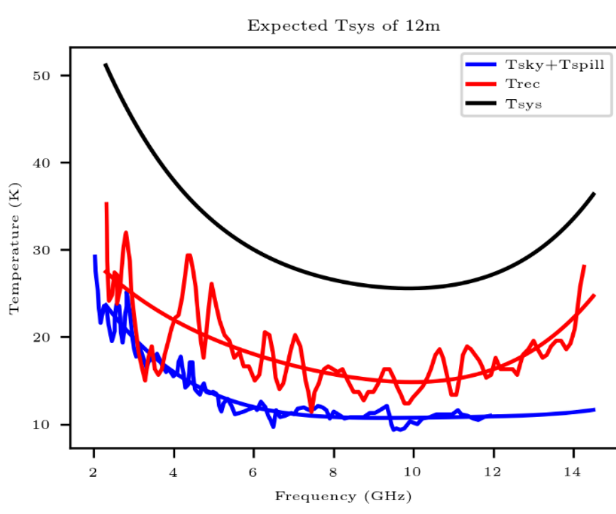
Figure 2: The expected system temperature ( T_{sys} ), receiver temperature ( T_{rec} ) and sky+spillover temperature as a function of frequency are shown. The expected values are obtained from laboratory measurements or calculations using similar system.
