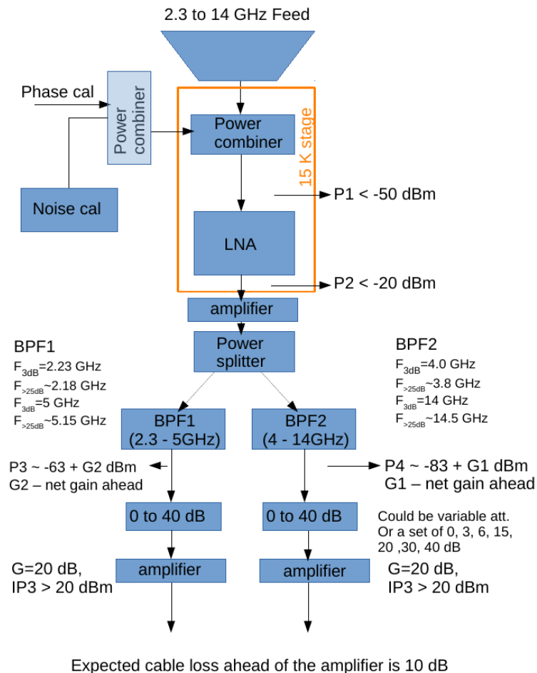
Figure 1. Block diagram of the cryogenic front-end system required for the 12m telescope at the Arecibo Observatory. Only one of the two polarizations are shown in the block diagram.
