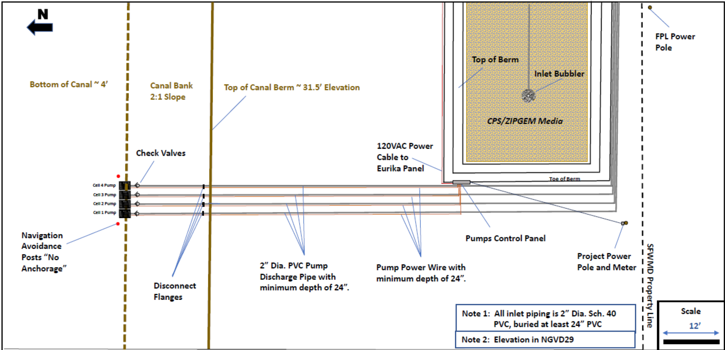
Sheet 11. Pump and Pipeline Layout
