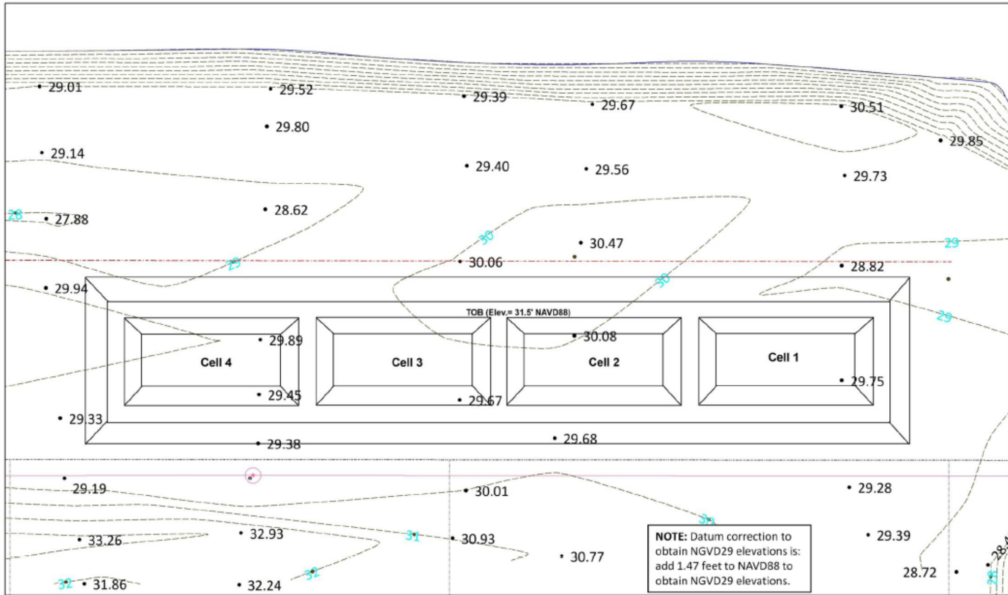
Sheet 3. Site Layout with Recent Topographical Survey (NAVD88) (Survey Completed by Altamax Surveying, Casselberry, FL) (See Datum correction note for NGVD29)
