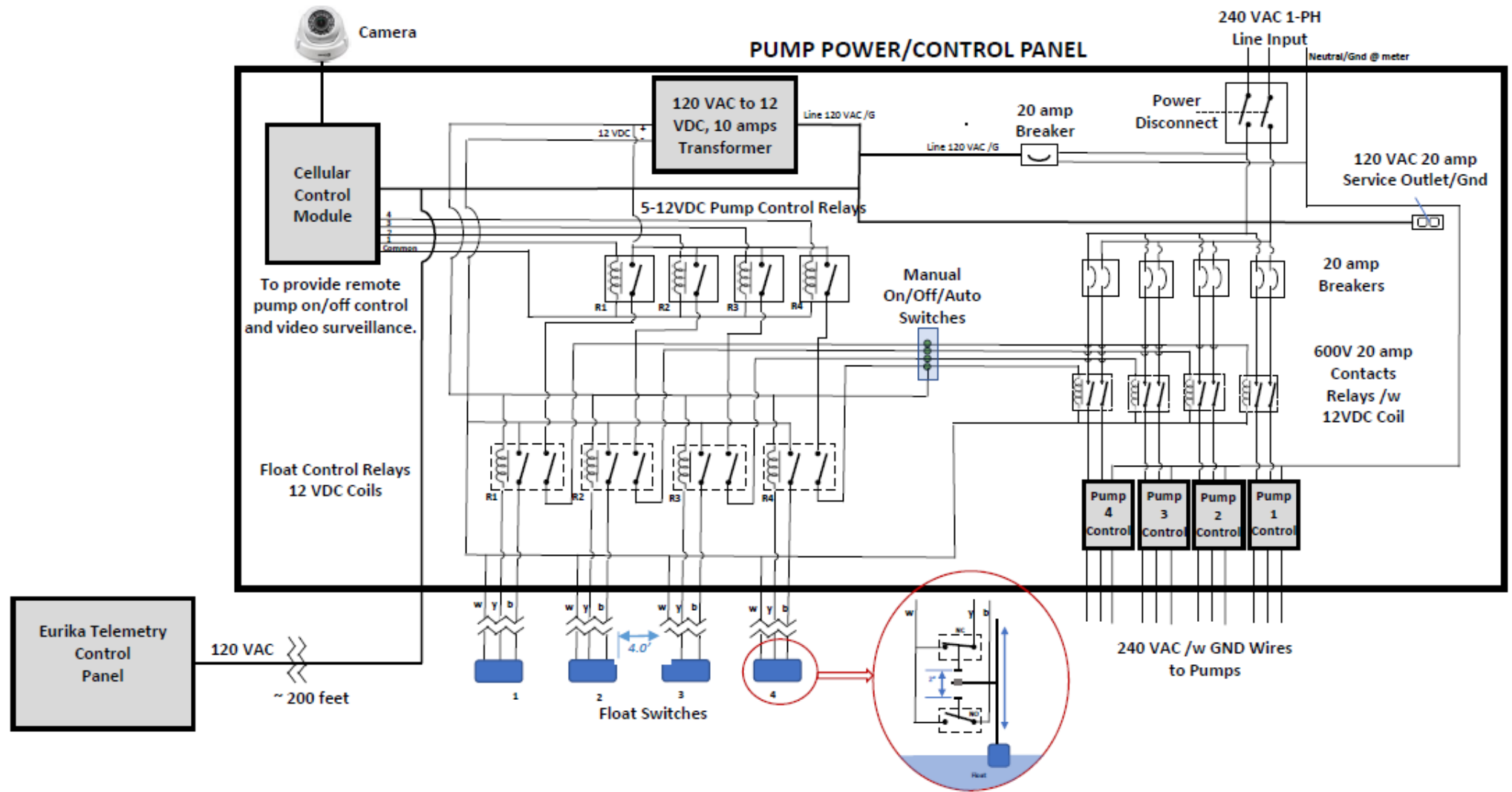
Sheet 12. Pump Power Control Panel with Pump Control Signals from Eureka Telemetry Panel
