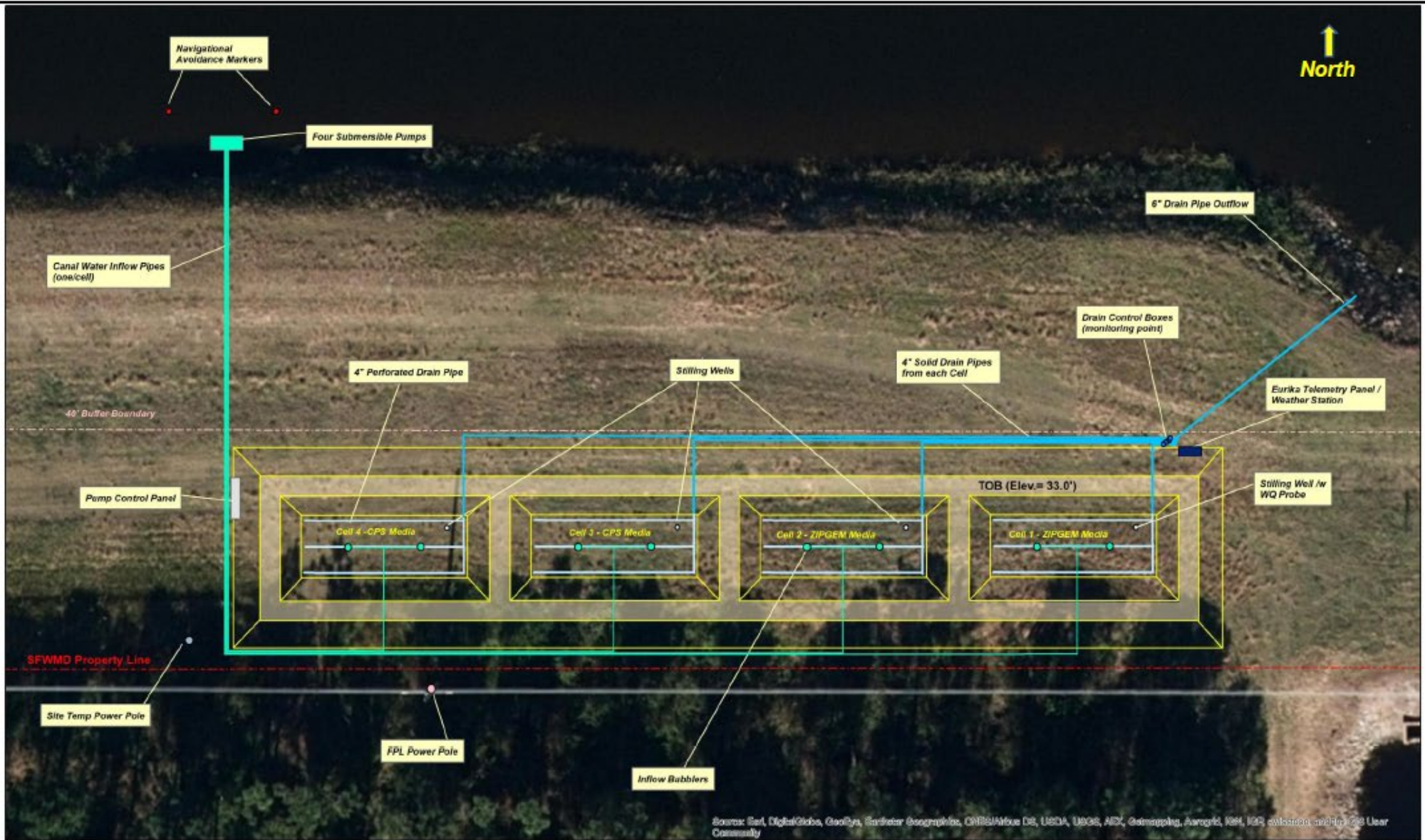
Sheet 2. General Layout of the C-23 Canal Bio-Sorption Activated Media Filtration to Reduce Nutrients and Algal Mass Project
