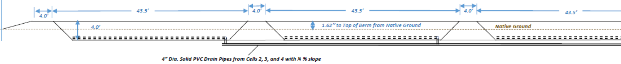
Sheet 4b. Infiltration Ponds Drainage Layout (Plan and North Profile View of Cells 2,
