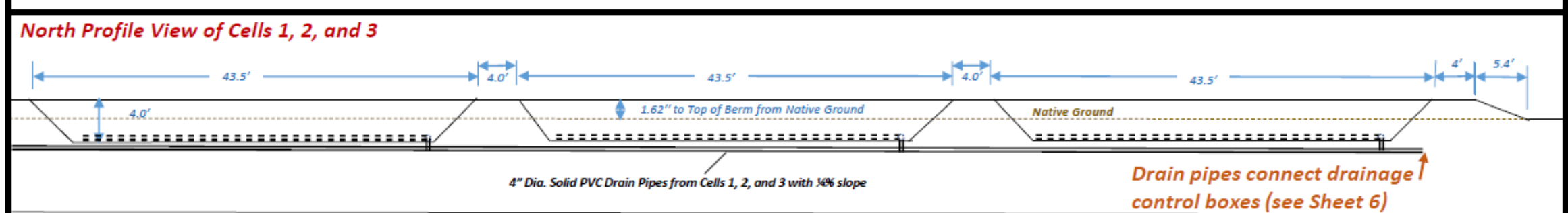
Sheet 4a. Infiltration Pond Layout (Plan and North Profile View of Cells 1, 2, and 3)
